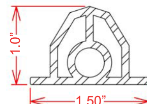
SMRP SECTION VIEW
